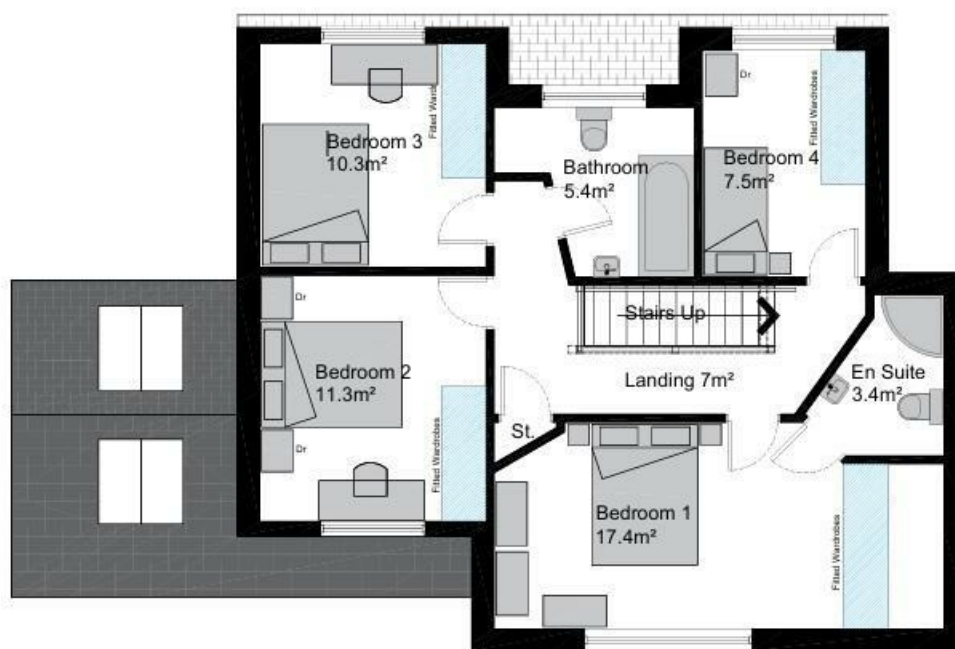
First Floor Layout 69m²
